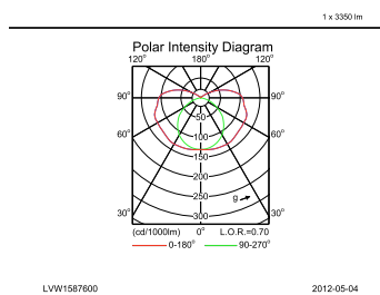
IFPC1_TCW060 1xTL-D36W HF.EPS
