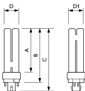
PL-C 26W/840/4P
