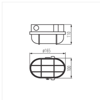
MILO 7040T/P
