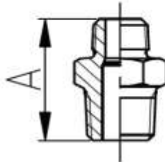
Reducing Nipple
