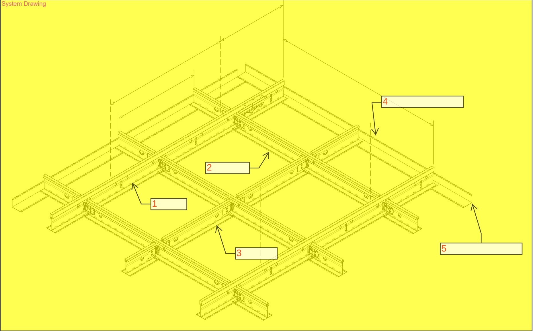
System Drawing
