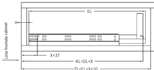
Sertar interior
