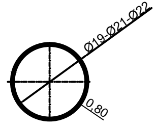
TUBE DETAIL
