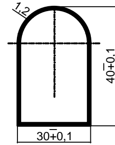
PROFILE DETAIL
