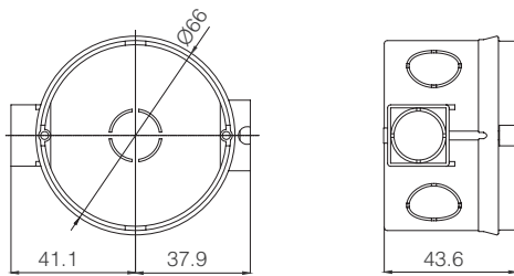
Plug-In Case for Under the Plaster
