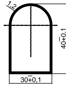
PROFILE DETAIL
