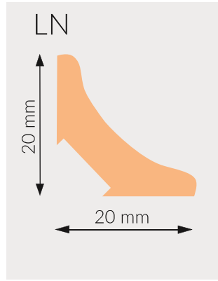
CORNER PROFILE
