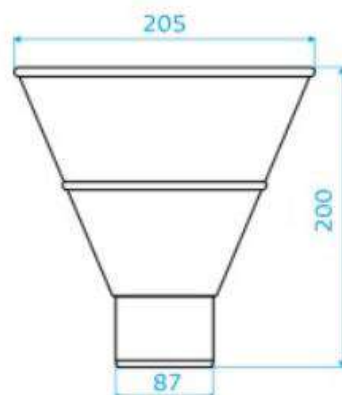
PĂLNIE Ø88MM
