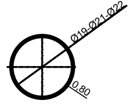
TUBE DETAIL
