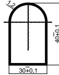
PROFILE DETAIL
