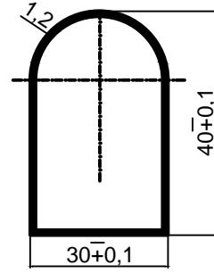
PROFILE DETAIL
