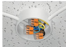
Lighting distribution in a ceiling canopy
