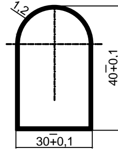
PROFILE DETAIL
