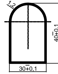
PROFILE DETAIL
