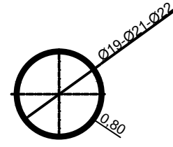
TUBE DETAIL
