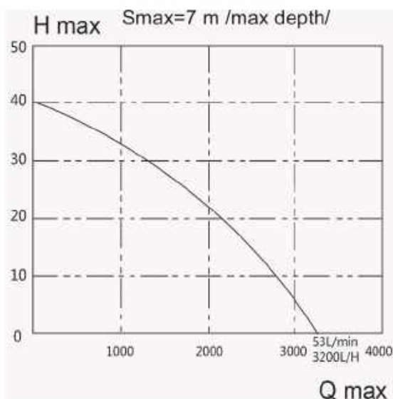
PUMP DIAGRAM
