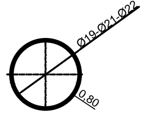
TUBE DETAIL
