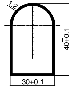
PROFILE DETAIL
