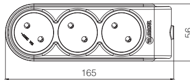
3 Gang Socket without Earthed
