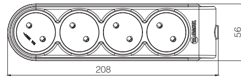
4 Gang Socket without Earthed
