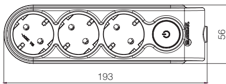
3 Gang Earthed Socket with Switch
